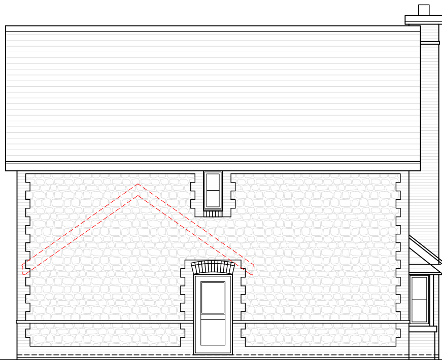
Rear Elevation
