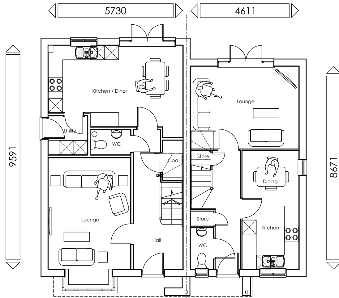
Ground Floor Plan Plot 26
