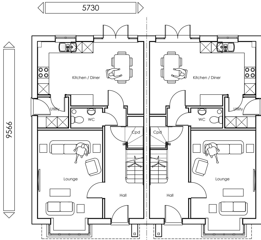
Ground Floor Plan Plot 31
