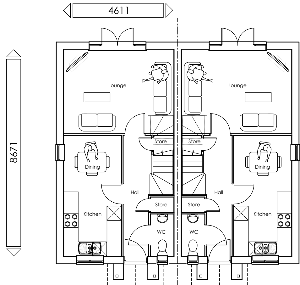
Ground Floor Plan Plot 3
