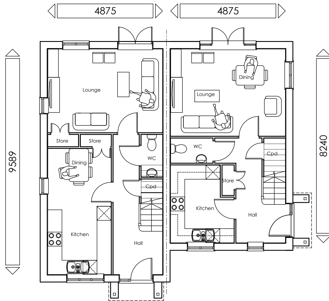
Ground Floor Plan Plot 20
