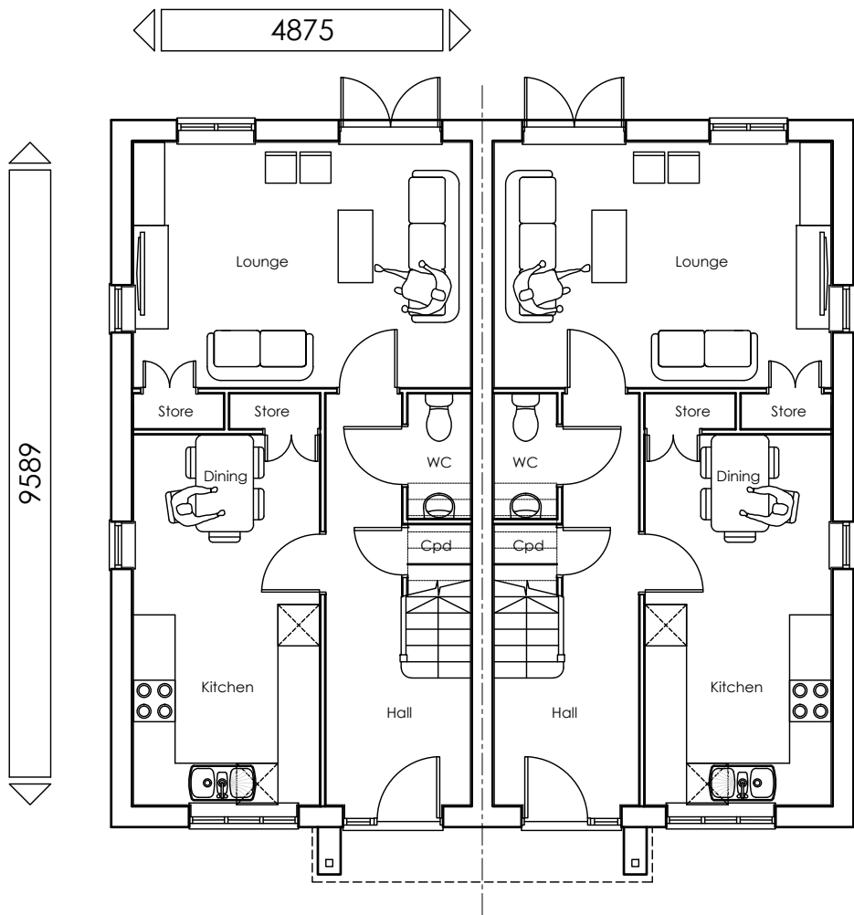
Ground Floor Plan Plot 9
