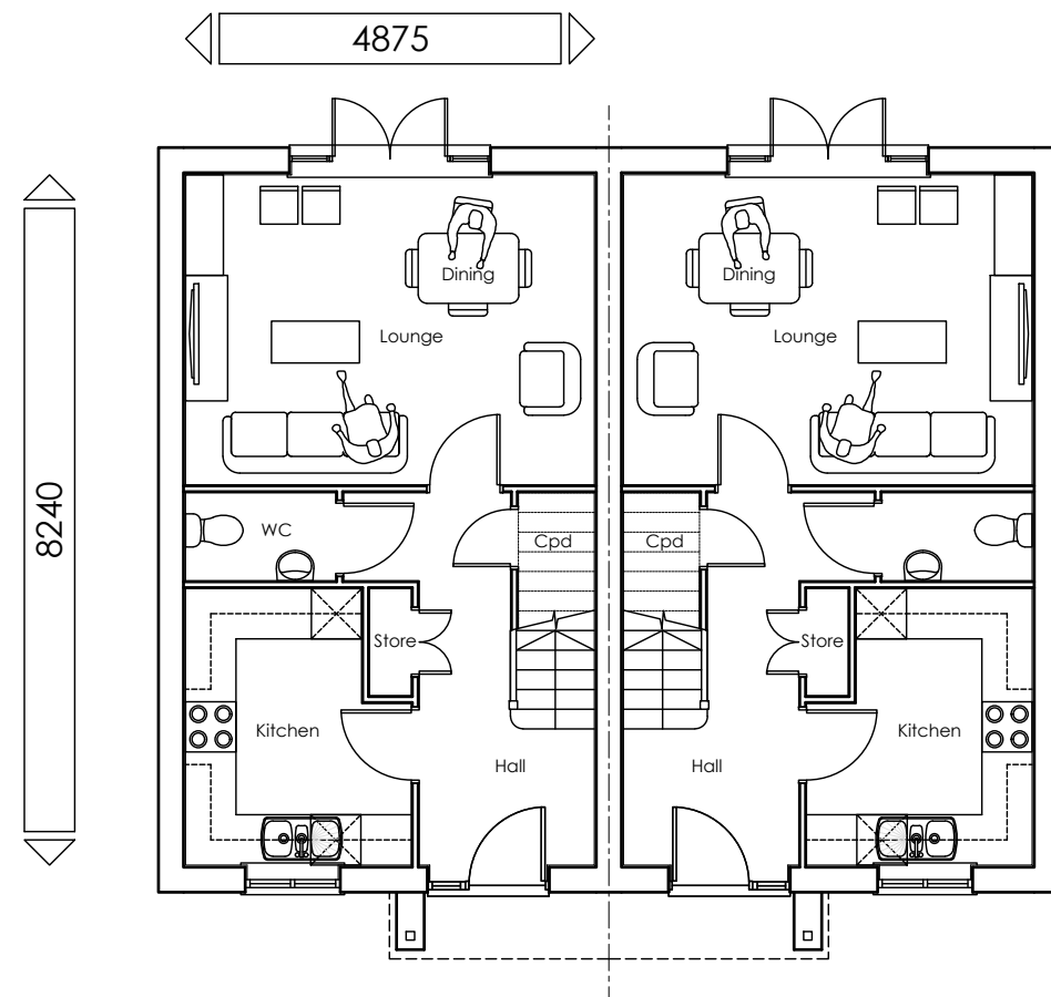
Ground Floor Plan Plots 18 & 22
